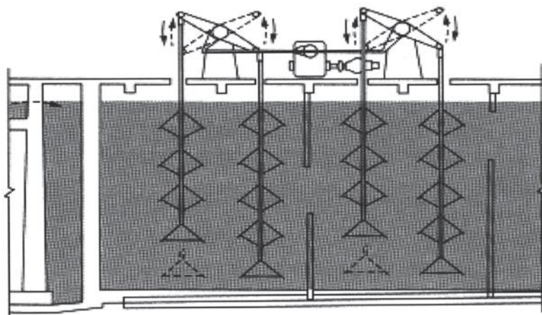
Walking-Beam Flocculator
