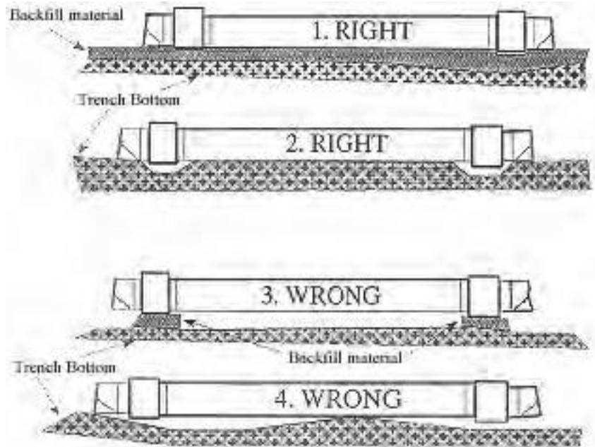
Figure 7.12 - Pipe Bedding
