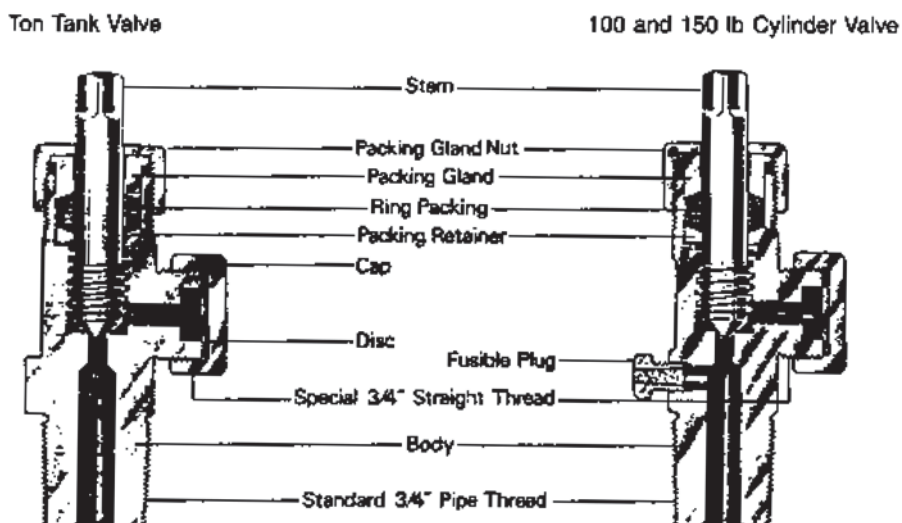
Figure 5.2 - Chlorine Cylinder Valve
