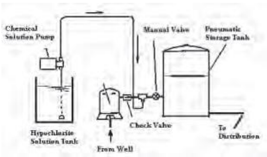
Figure 5.6 - Typical Hypochlorination System
