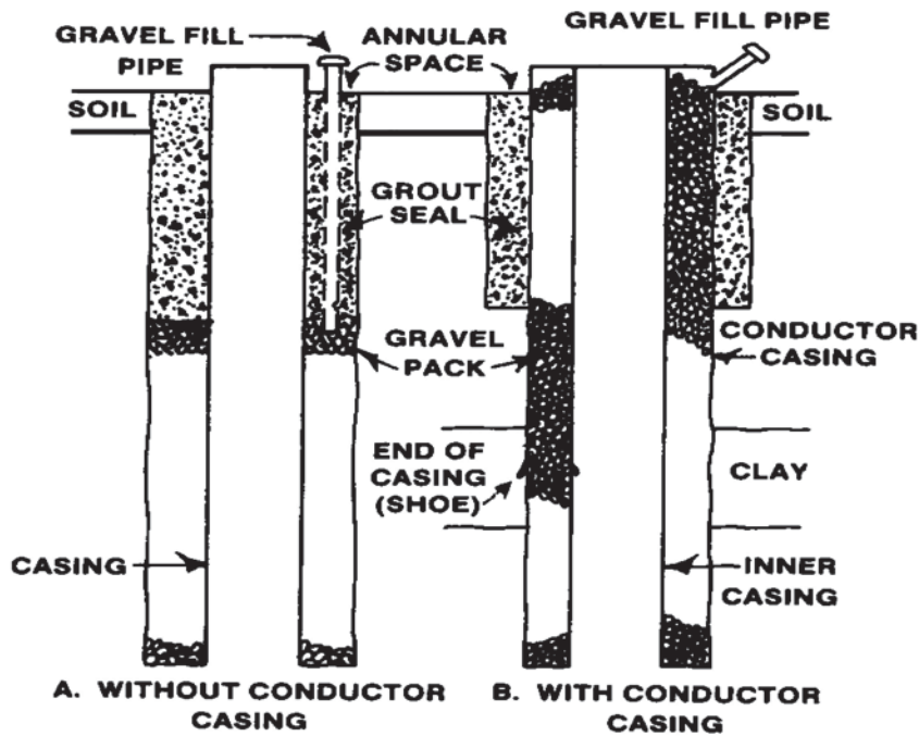
Figure 11.5 - Gravel Packed Well Types
