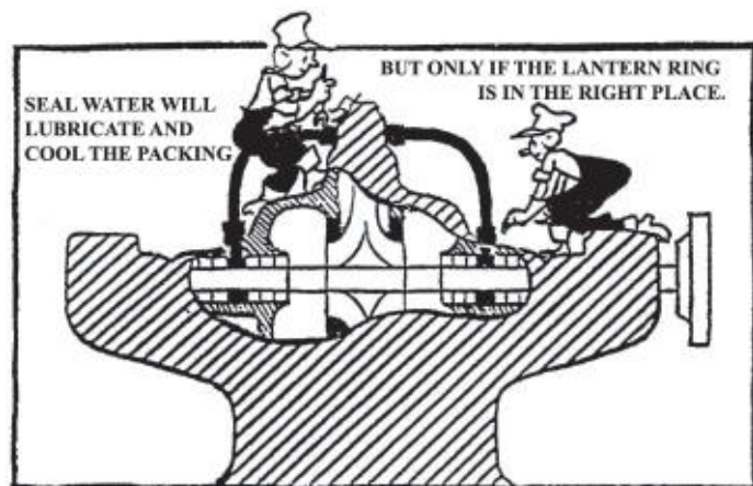
Figure 9.11 - Seal Water
