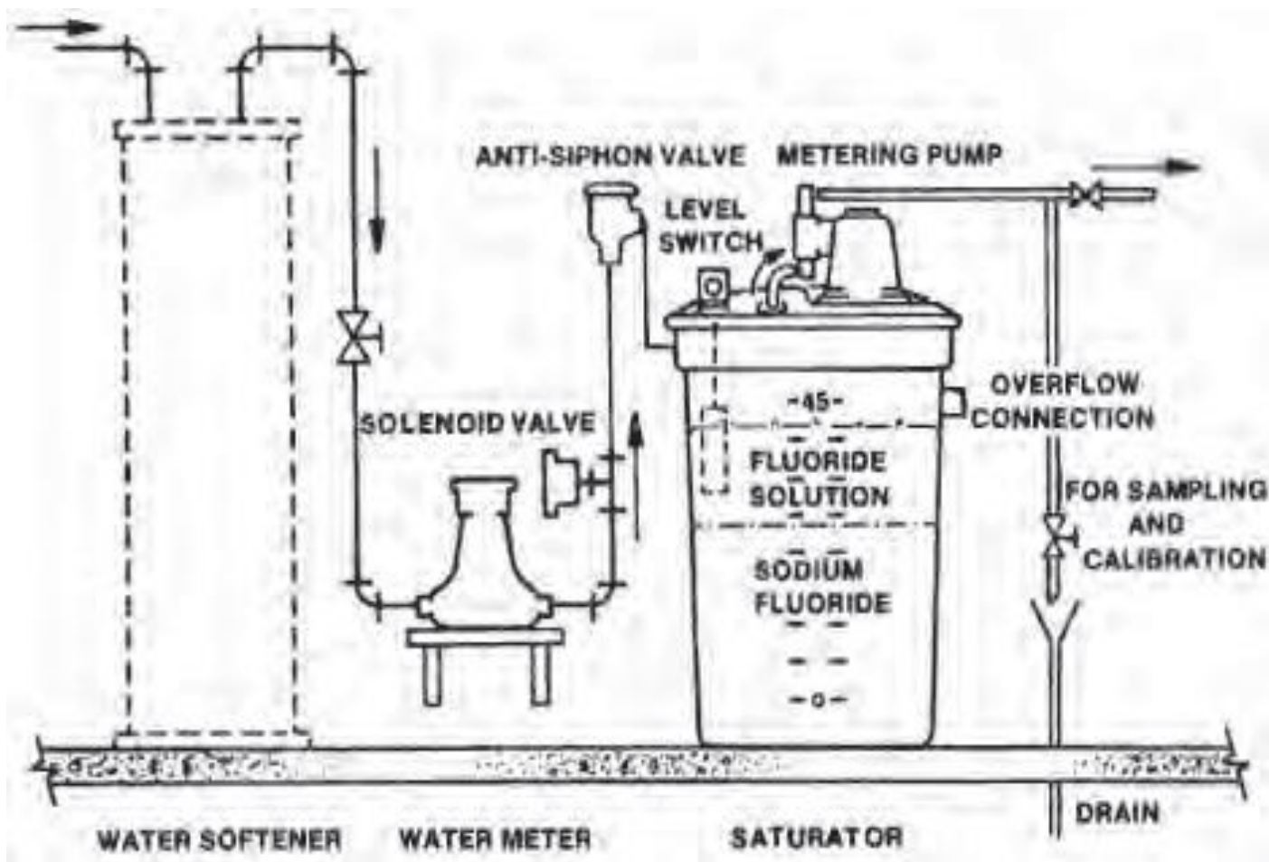
Figure 6.2 - Sodium Fluoride Saturator
