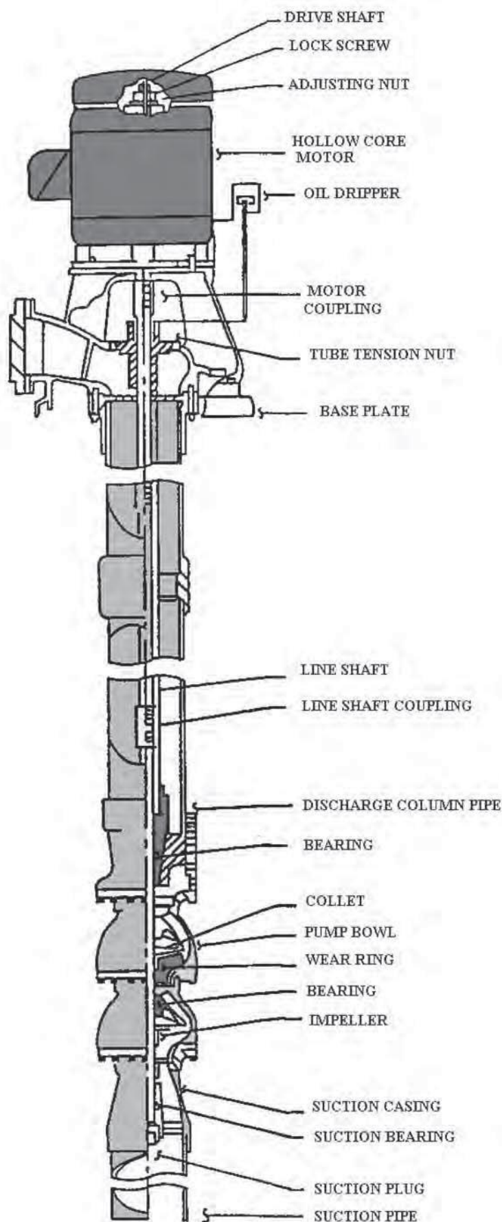
Figure 11.6 - Vertical Turbine Centrifugal Pump
