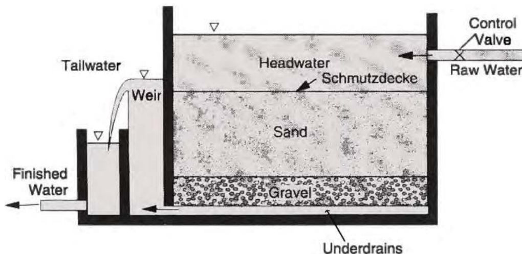
Figure 12.17 - Slow Sand Filter
