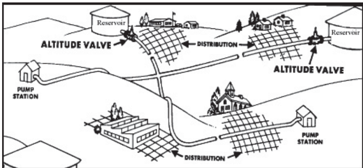
Figure 7.17 - Altitude Valve
