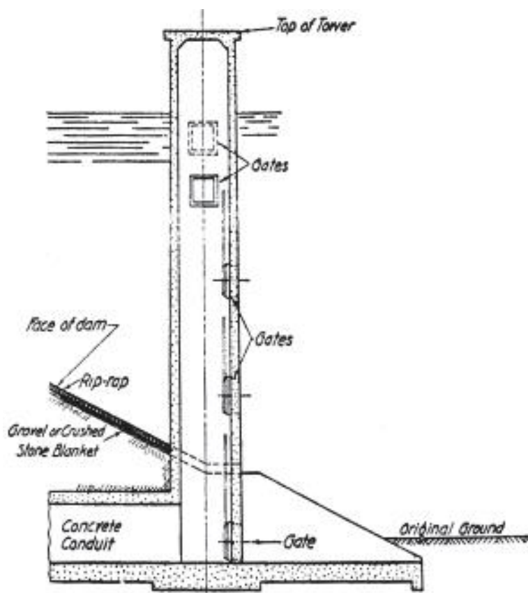
Figure 12.1 - Lake Intake Structure
