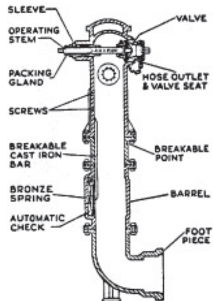
Wet Barrel Hydrant
