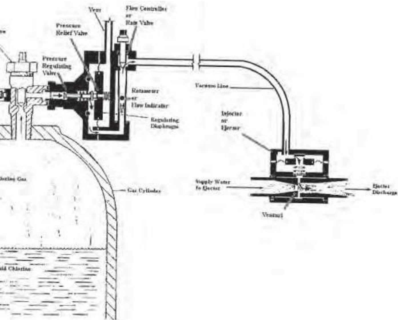
Figure 5.5 - 150 lb Chlorine Gas Feed Unit
