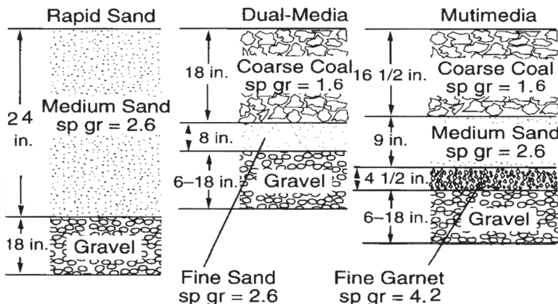
Figure 12.23 - Filter Media Configurations
