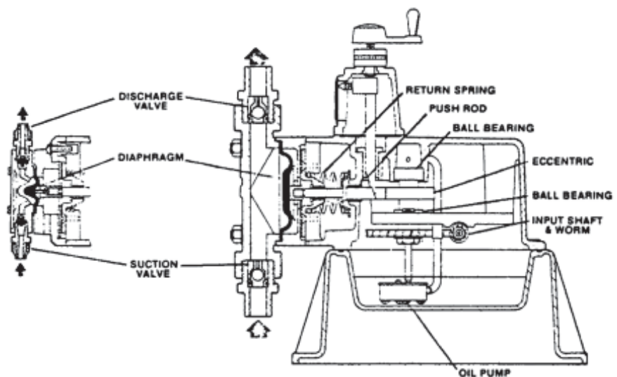
Figure 10.9 - Diaphragm Pump
