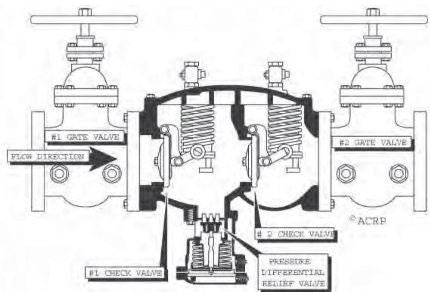
Figure 7.28 - RPZ Device
