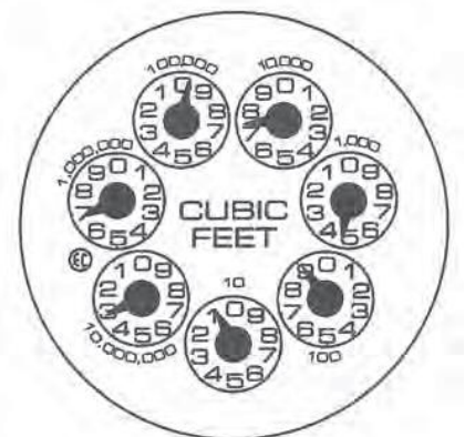
Figure 7.21 - Water Meter Dial
