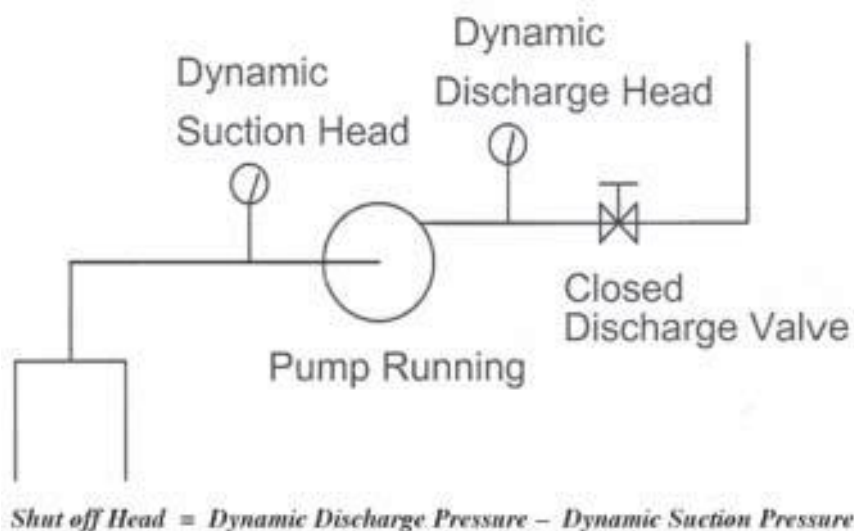
Figure 9.16 - How to Determine Shut-Off Head
