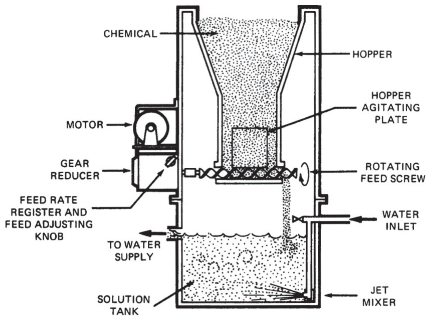
Figure 10.7 - Volumetric Chemical Feeder
