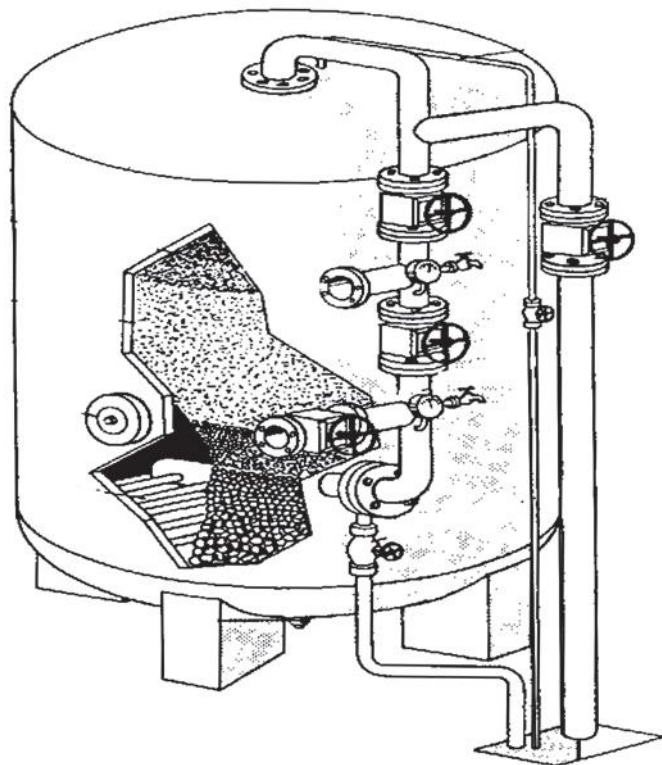
Figure 12.16 - Pressure Filter
