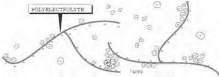
Figure 12.7 - Polyelectrolyte
