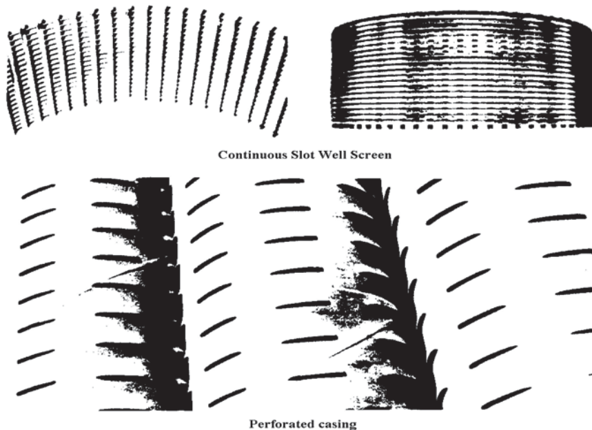
Figure 11.8 - Well Screens
