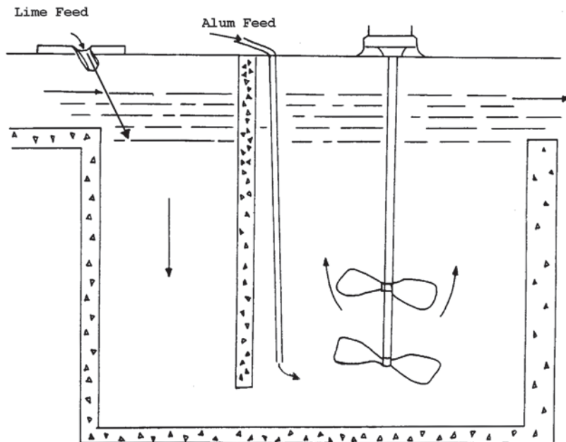
Figure 12.10 - Dual Compartment Rapid Mix
