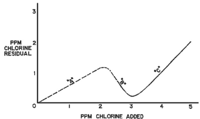
Figure 5.1 - Breakpoint Curve
