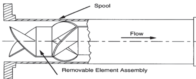
Figure 12.9 - Static In-Line Mixer
