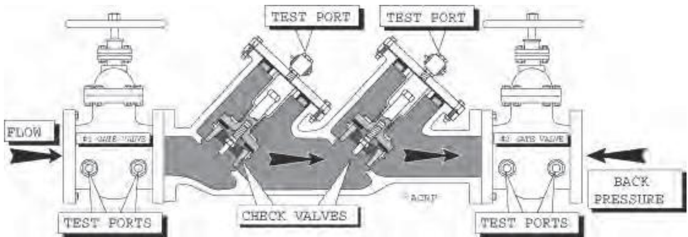
Figure 7.27 - Double Check Valve
