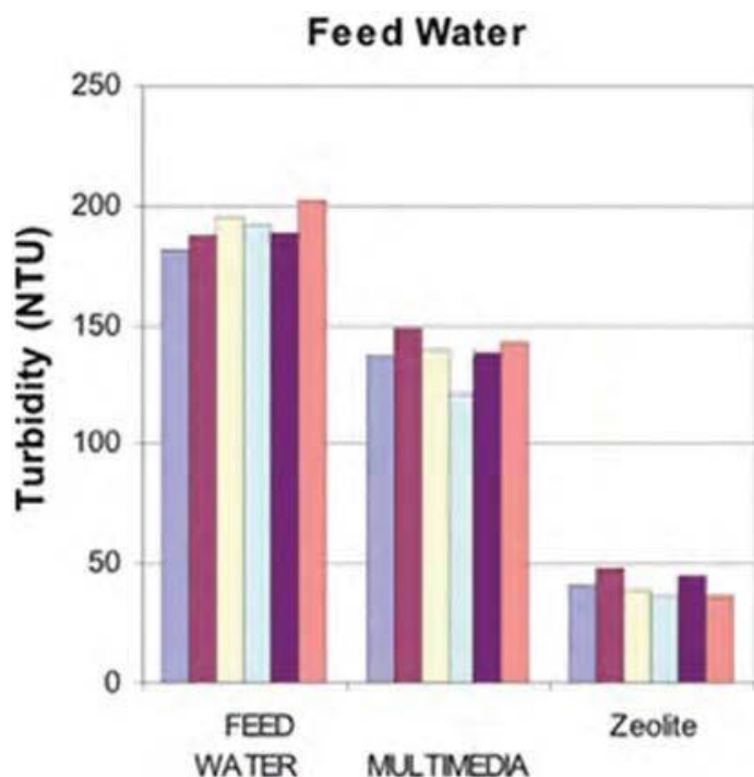
Figure 15.7 - Turbidity Rates in Various Media
