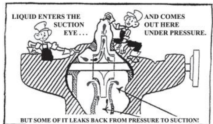
Figure 9.9 - Leak Back
