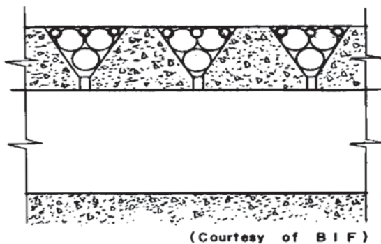
Figure 12.19 - Wheeler Filter Block
