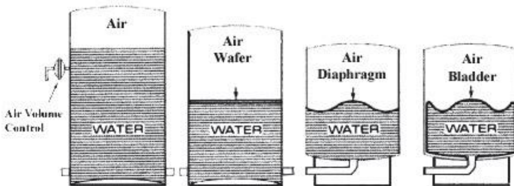
Figure 8.2 - Types of Pneumatic Tanks
