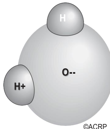
Figure 3.2 - Water Molecule
