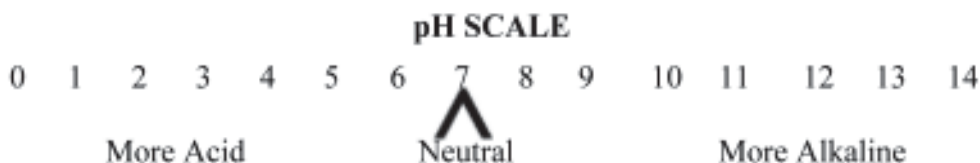
Figure 12.2 - pH Scale
