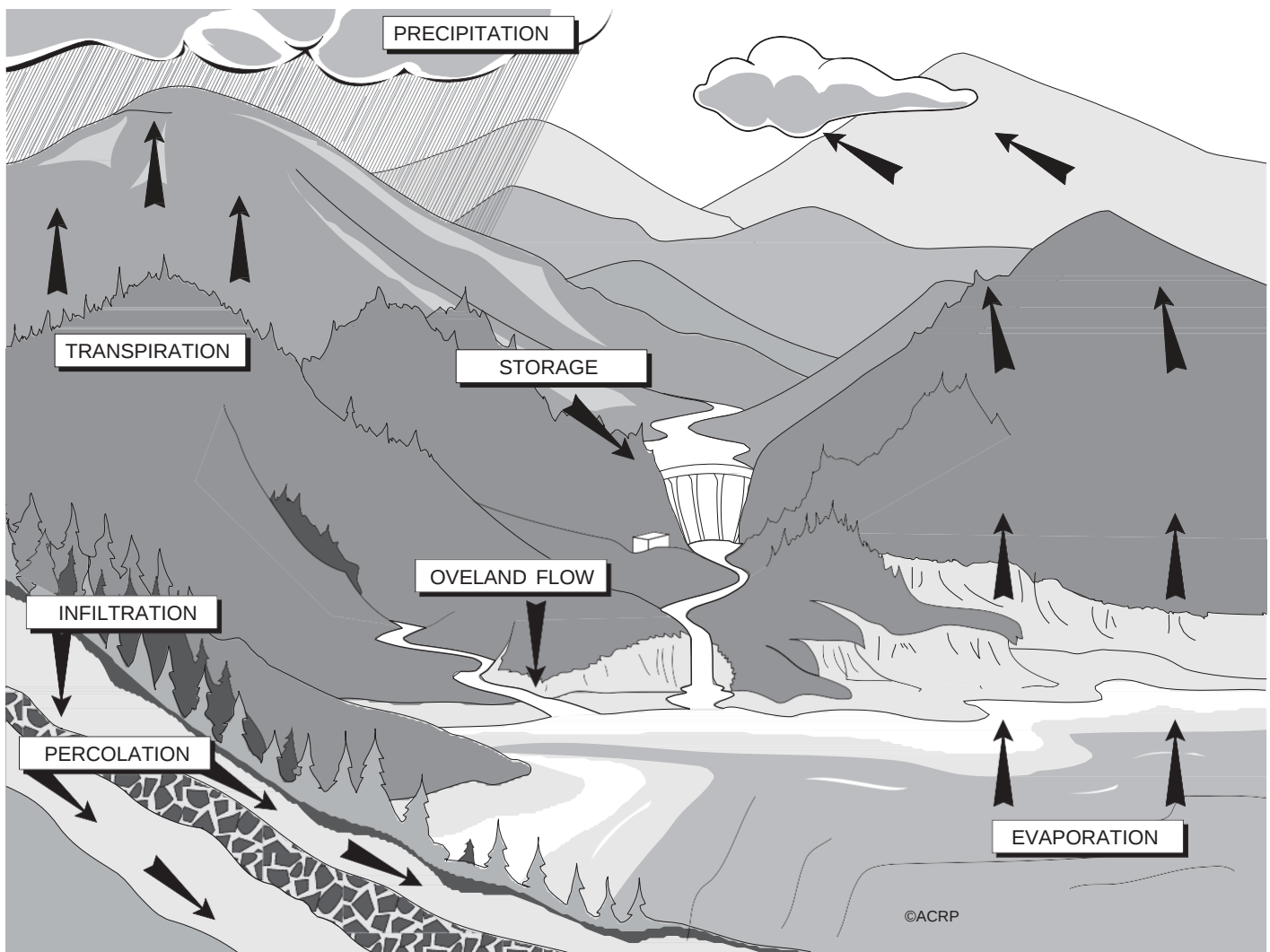
Figure 3.3 - The Hydrologic Cycle
