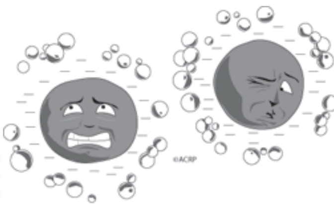
Figure 12.4 - Hydrophobic Particles
