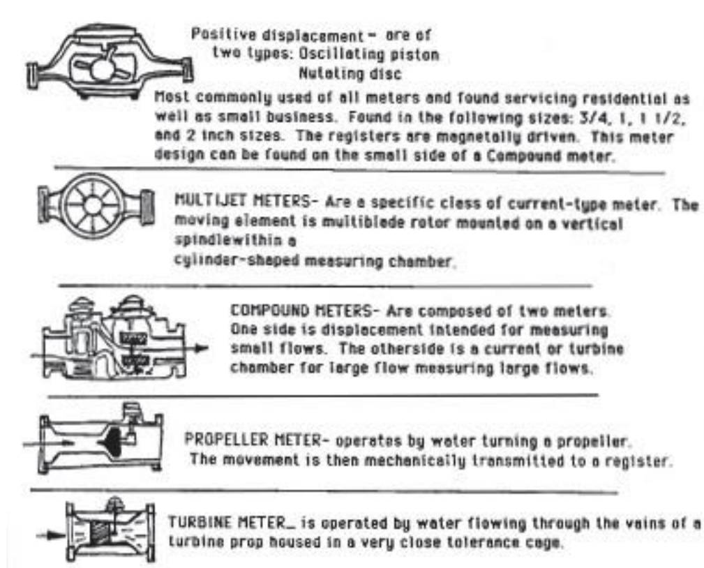
Figure 7.20 - Types of Meters
