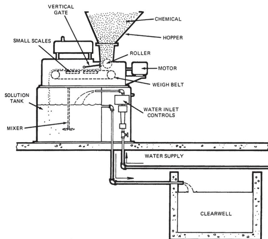
Figure 10.6 - Gravimetric Chemical Feeder
