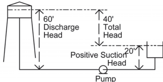
Figure 9.14 - How to Determine Total Head
