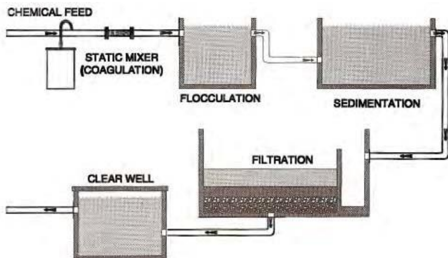
Figure 12.3 - Conventional Water Treatment Plant Diagram
