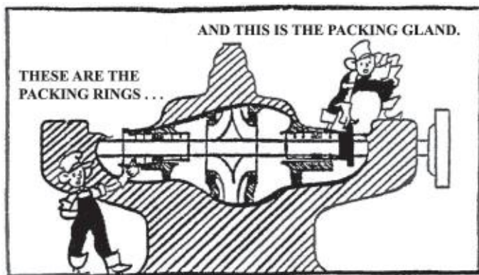
Figure 9.10 - Stuffing Material
