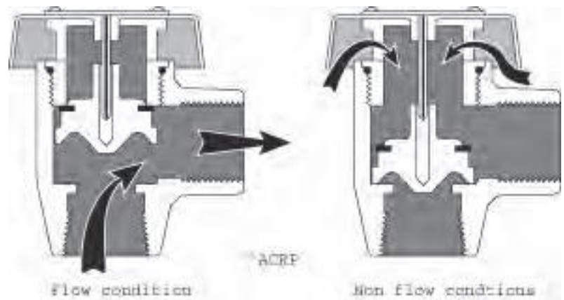
Figure 7.26 - Atmospheric vacuum breaker
