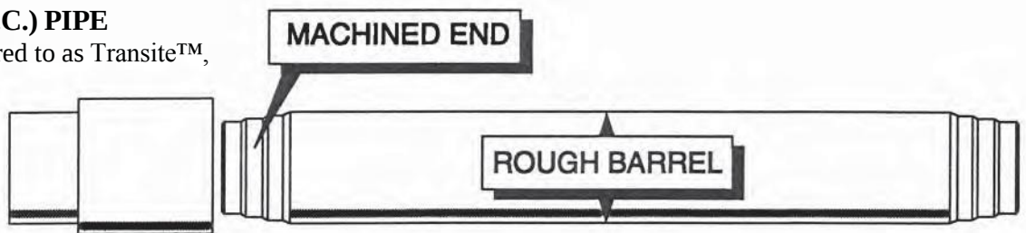
Figure 7.4 - Asbestos Cement (A.C.) Pipe
