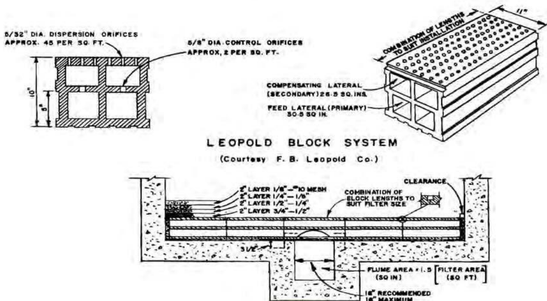
Figure 12.18 - Filter Underdrain System
