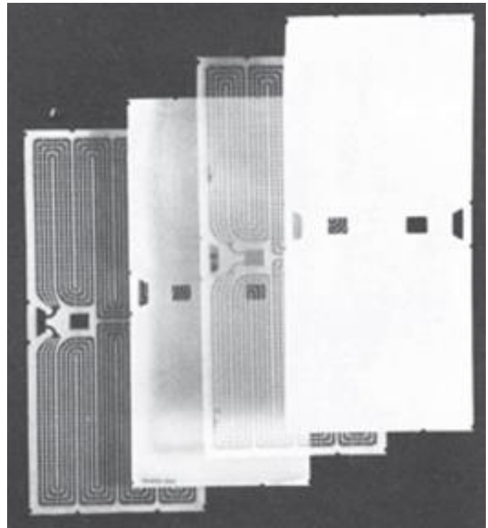
Figure 15.21 - Cell pair: Spacer, Cation Membrane, Spacer, Anion Membrane (courtesy Ionics)
