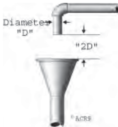
Figure 7.25 - Air Gap
