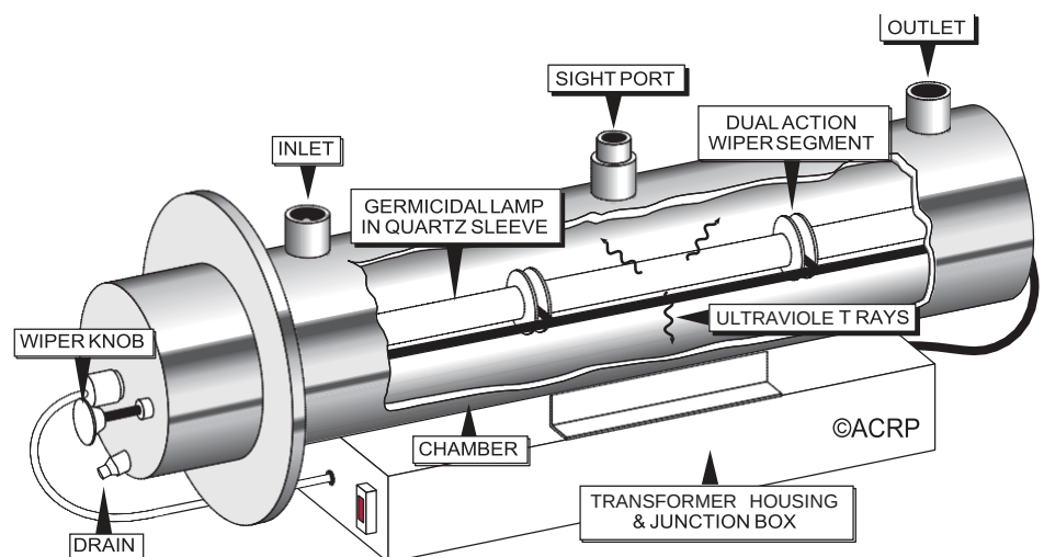
Figure 5.7 - UV Disinfection System
