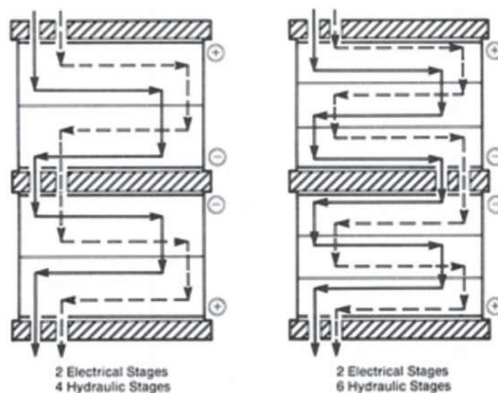
Figure 15.23 - ED Stack Hydraulic and Electrical Stages (courtesy Ionics)
