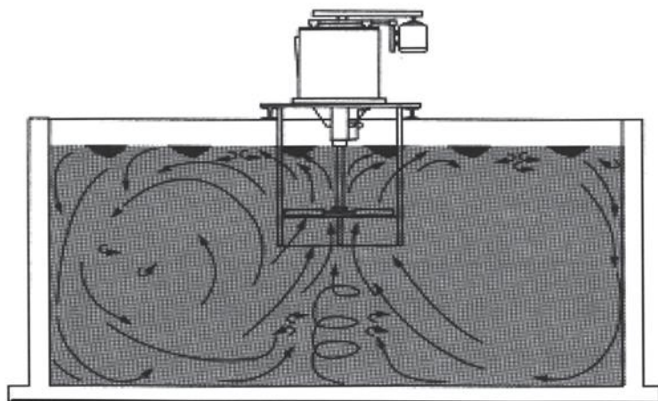
Turbine Flocculator
