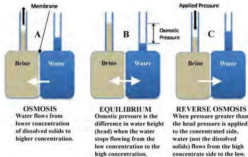
Figure 15.18 a,b,c - Reverse Osmosis Principle
