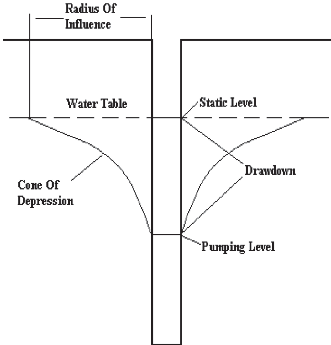
Figure 11.9 - Water Well Hydraulic Terms
