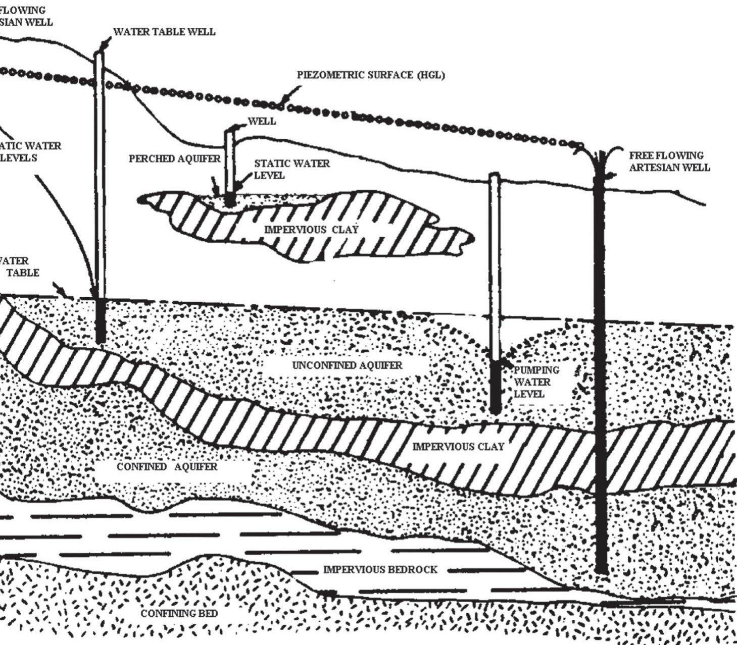
Figure 11.2 - Artesian & Water Table Aquifers
