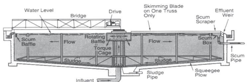
Figure 12.14 - Circular Sedimentation Basin
