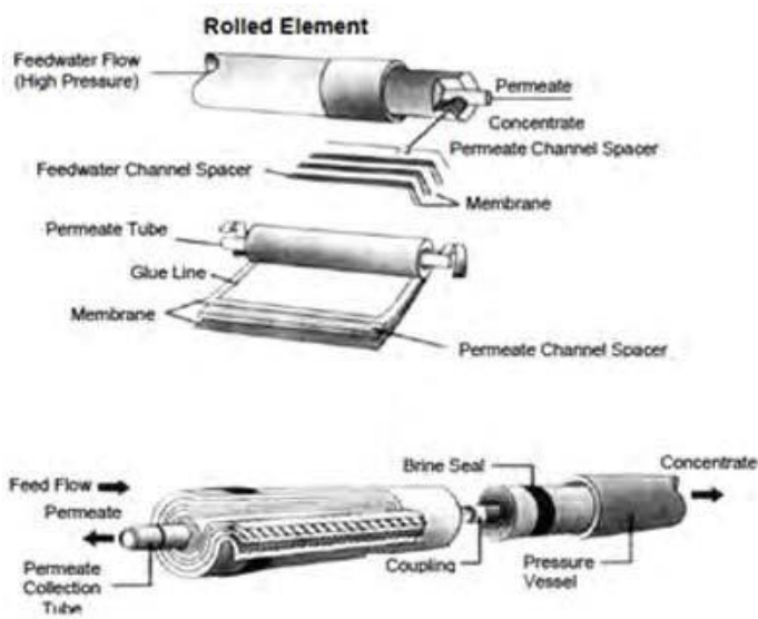
Figure 15.11 - Construction of FilmTec RO membrane element (DOW/Filmtec Product Sheet) [1]
