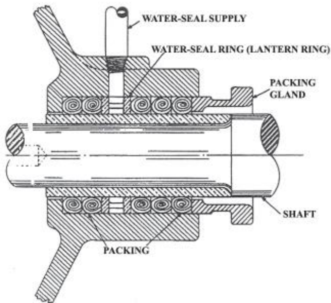
Figure 9.12 - Stuffing Box Cross-Section
