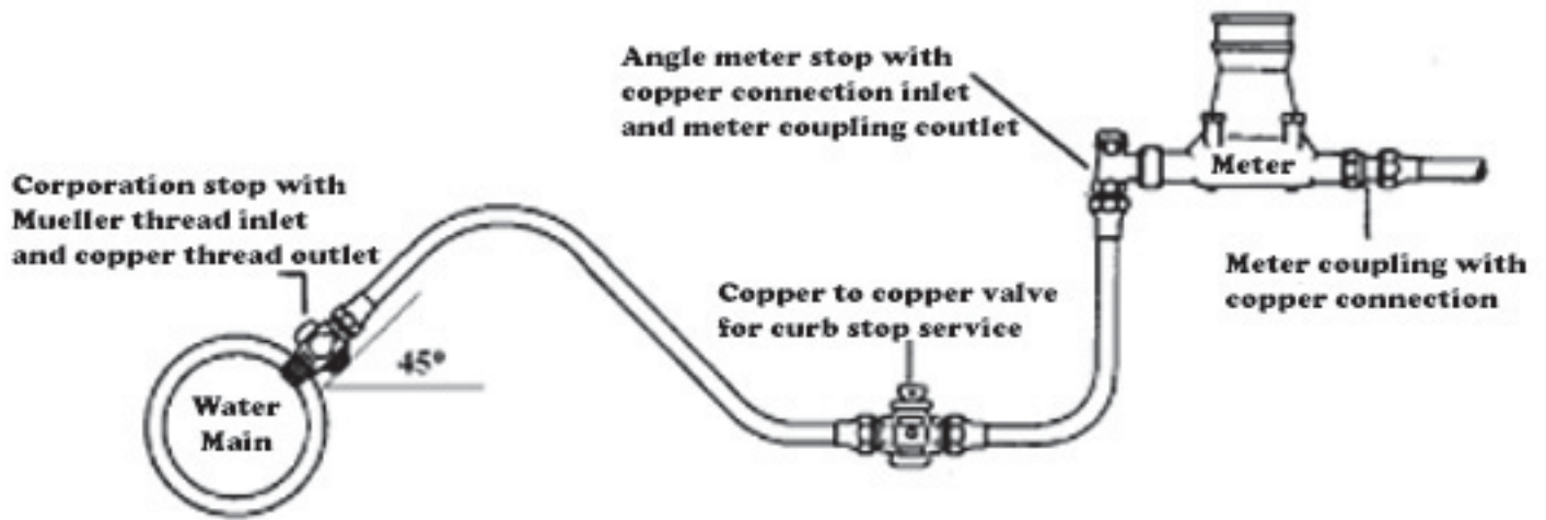
Figure 7.19 - Service Line Installation
