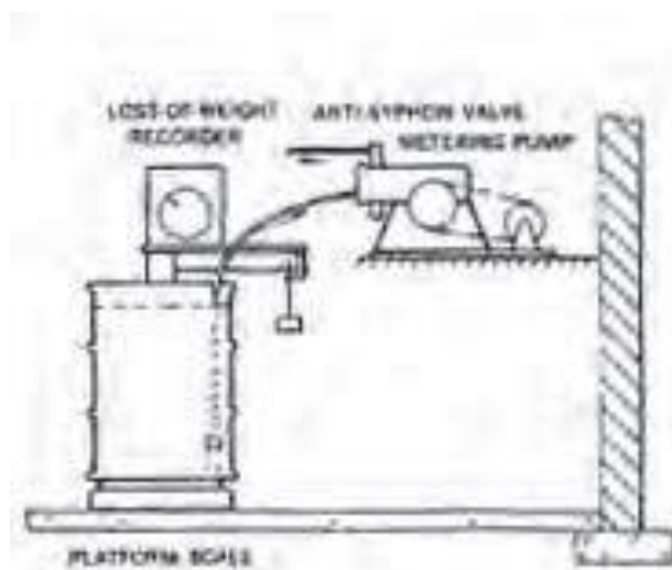
Direct Acid Feed System
