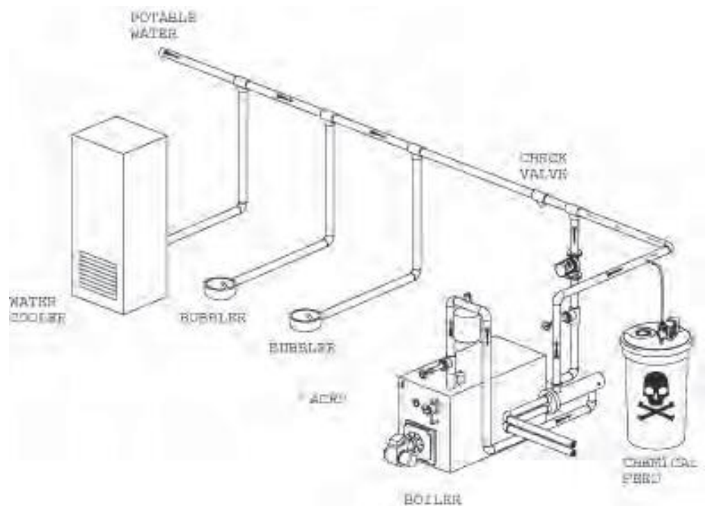
Figure 7.24 - Backpressure with boilers
