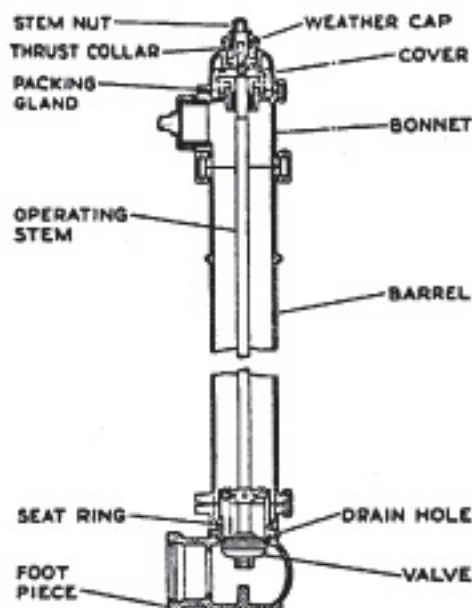
Dry Barrel Hydrant
