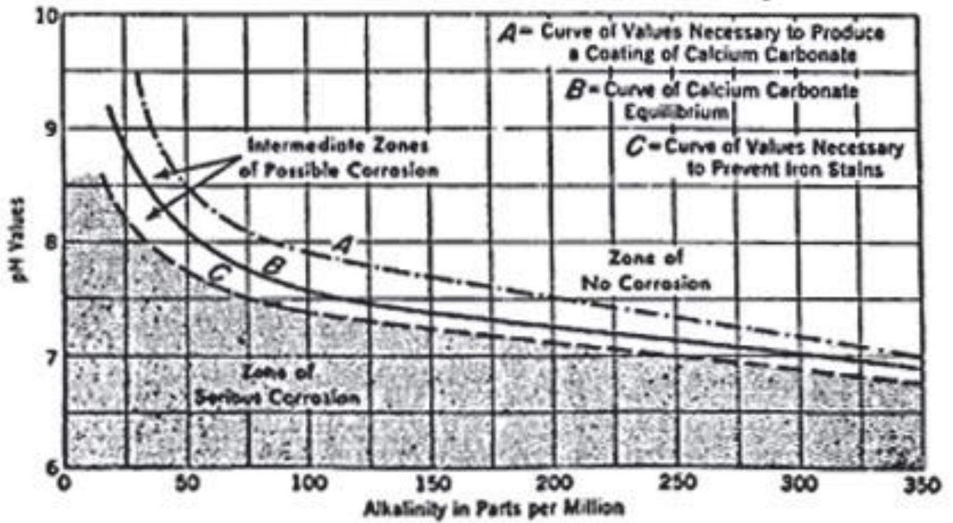
Figure 7.23 - Baylis Curve
