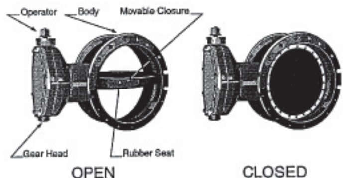
Figure 7.16 - Butterfly Valve
