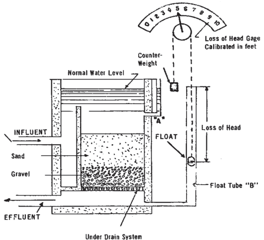
Figure 12.20 - Loss of Head Gauge 12-19
