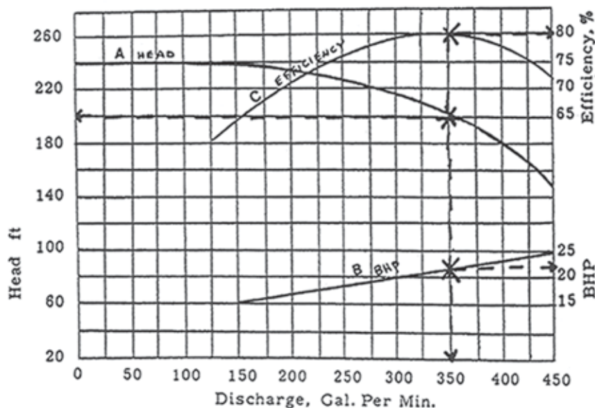
Figure 9.15 - Pump Curve
