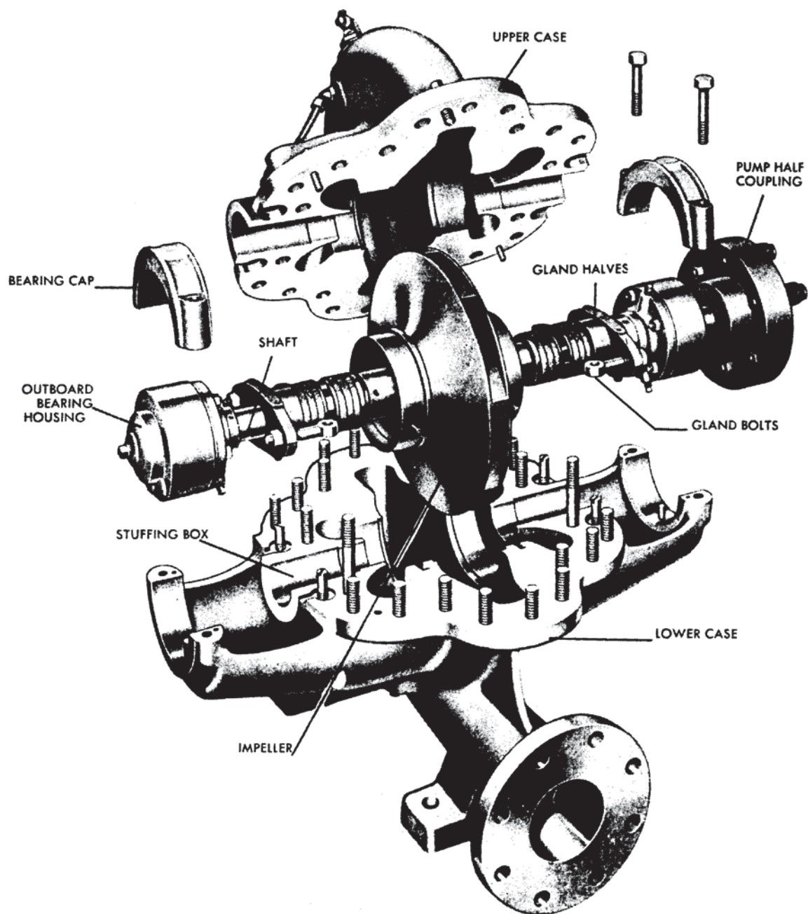
Figure 9.2 - Horizontal Split Case Centrifugal Pump
