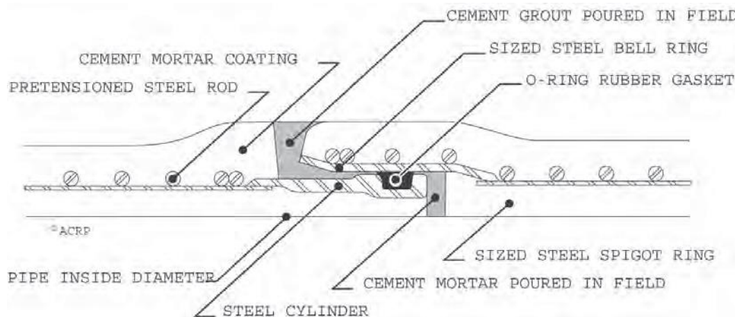
Figure 7.10 - Cross-section of Pretensioned Concrete Cylinder Pipe Joint
