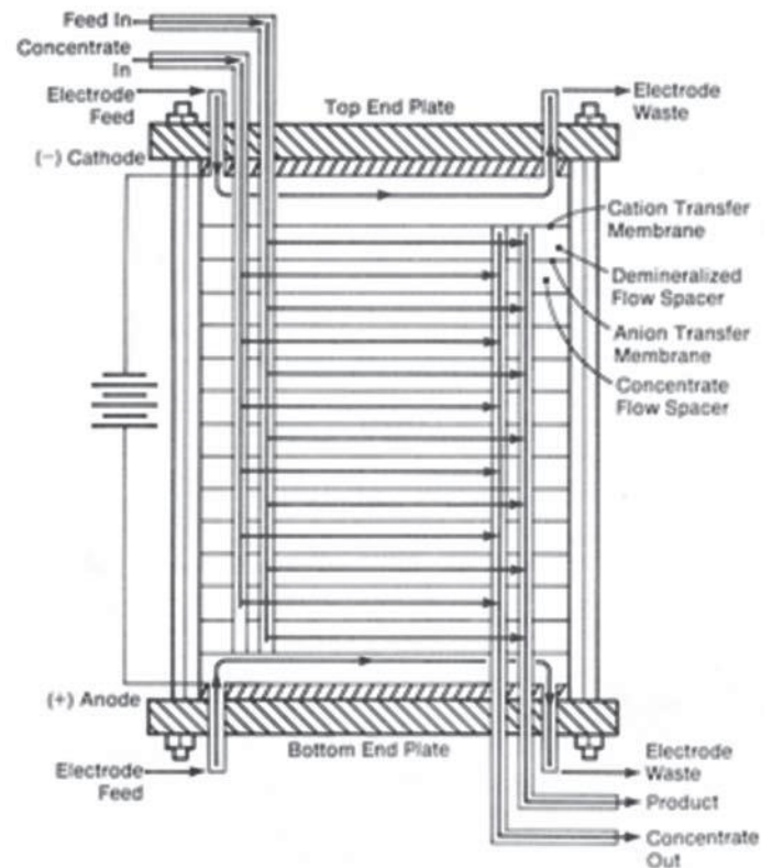
Figure 15.22 - ED Stack Flow Path (courtesy Ionics)
