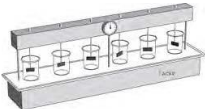
Figure 12.8 - Jar Test Apparatus
