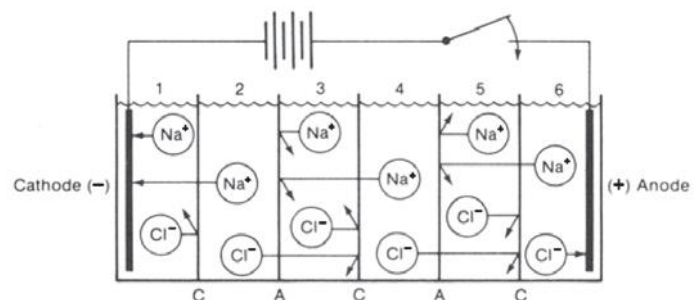
Figure 15.20 - ED Stack Demineralization Compartments (courtesy Ionics)
