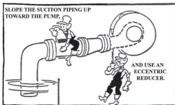
Figure 9.8 - Suction Piping
