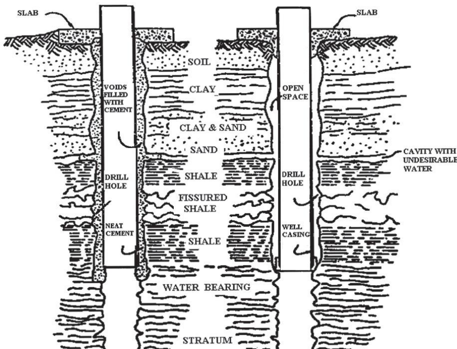
Figure 11.3 - Grouting A Well Casing
