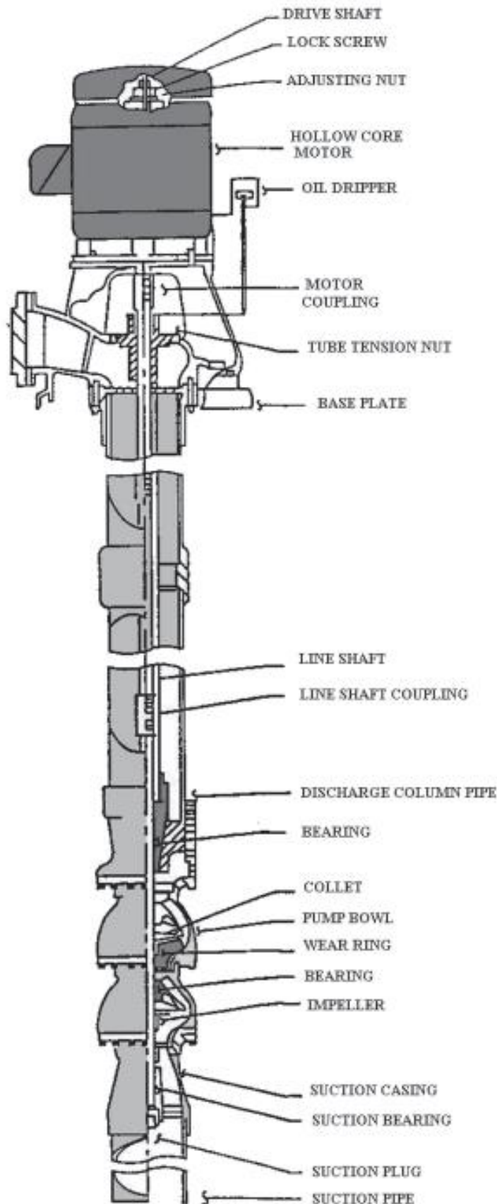
Figure 9.4 - Vertical Turbine Centrifugal Pump
