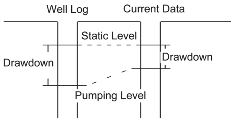
Figure 11.13 - Well Problem - Mechanical Pump
