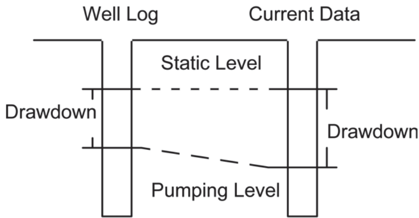
Figure 11.11 - Well Problem - Clogged Screen
