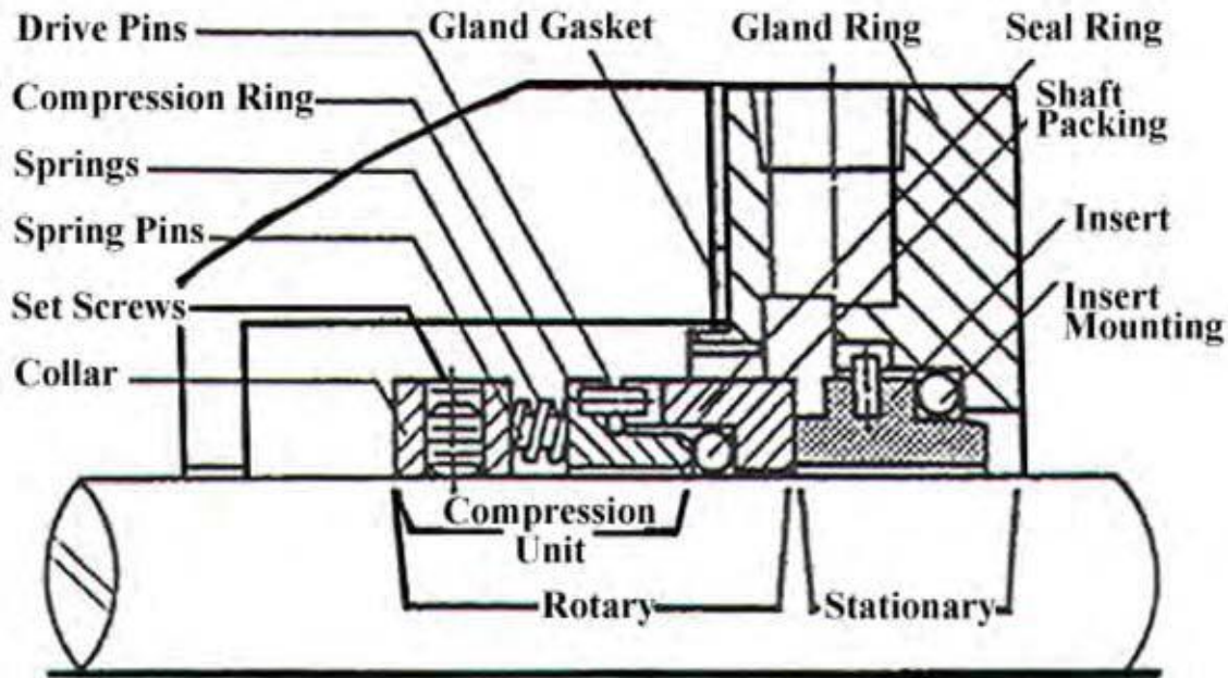
Figure 9.13 - Mechanical Seal Components
