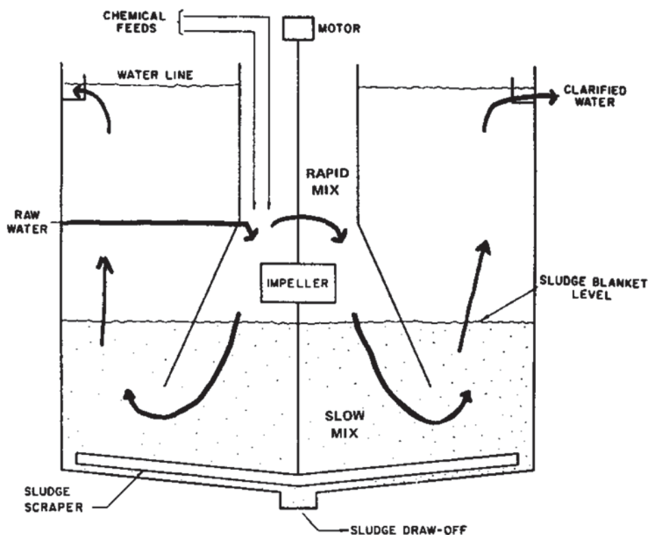
Figure 12.15 - Up-Flow Clarifier
