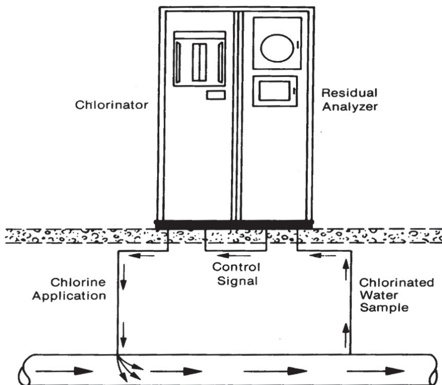
Figure 10.5 - Feedback Control Loop
