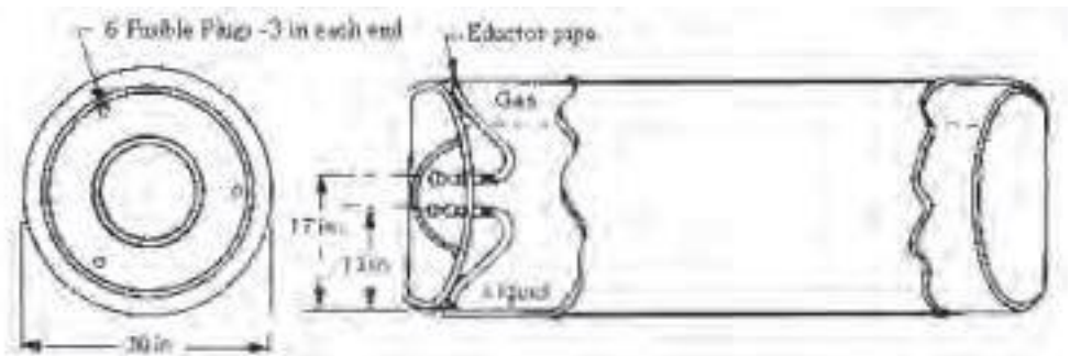
Figure 5.4 - Cross Section of a 1-ton Cylinder
