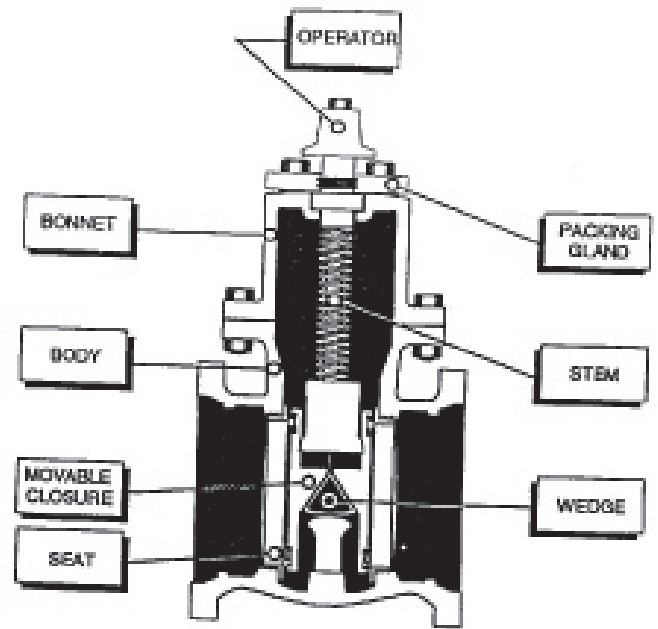
Figure 7.15 - Non-Rising Stem Gate Valve
