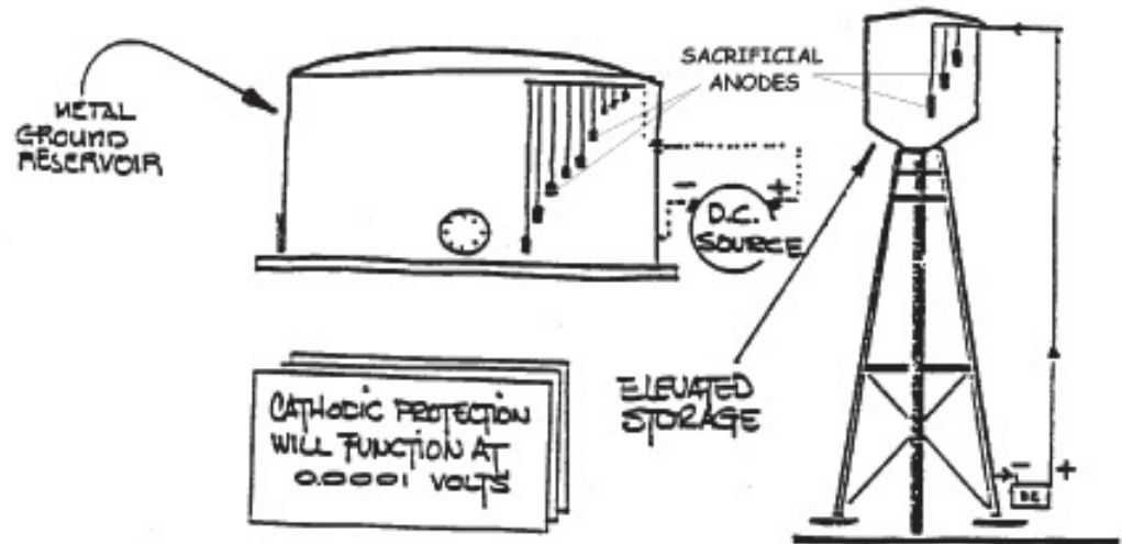
Figure 8.1 - Sacrificial Anodes Used for Cathodic Protection
