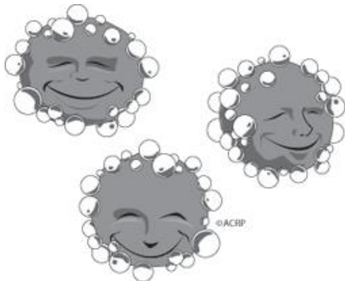
Figure 12.5 - Hydrophilic Particles
