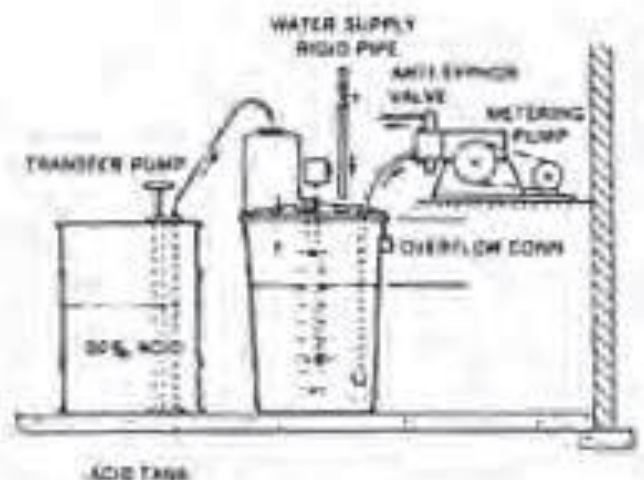
Diluted Acid Feed System
