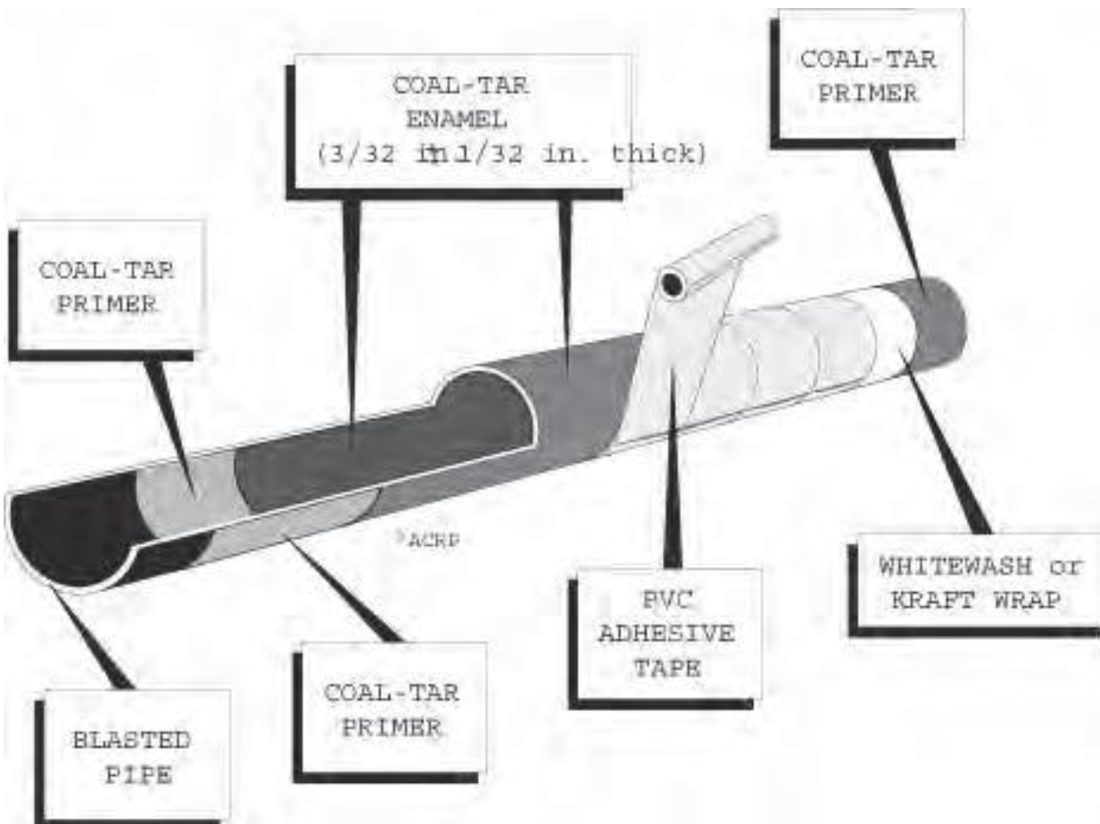
Figure 7.7 - Steel Pipe, dipped and wrapped
