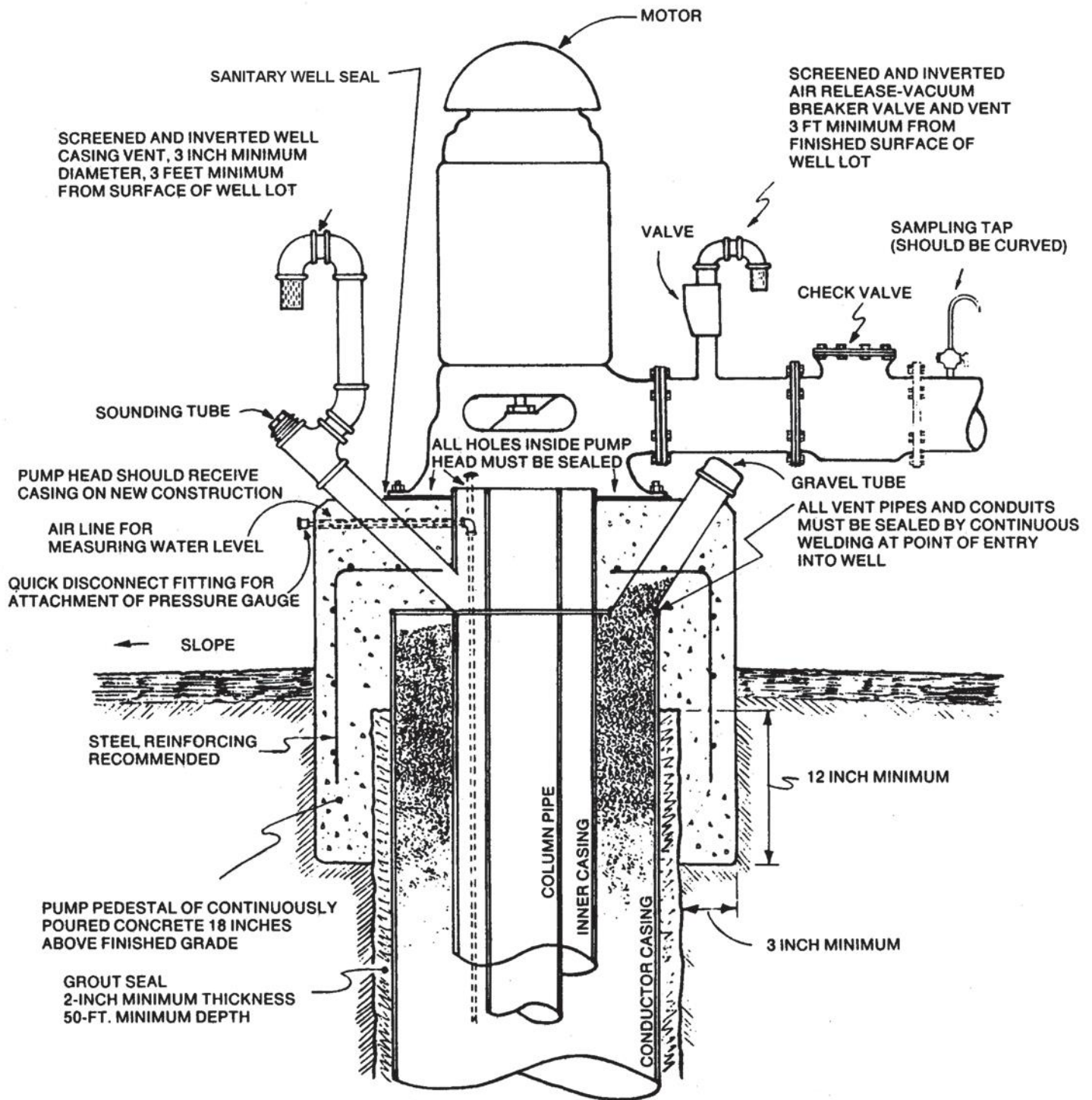
Figure 11.4 - Gravel Pack Well Construction
