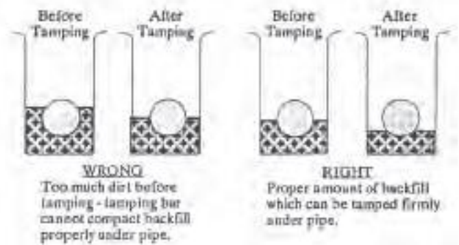
Figure 7.13 - Backfilling the Pipe
