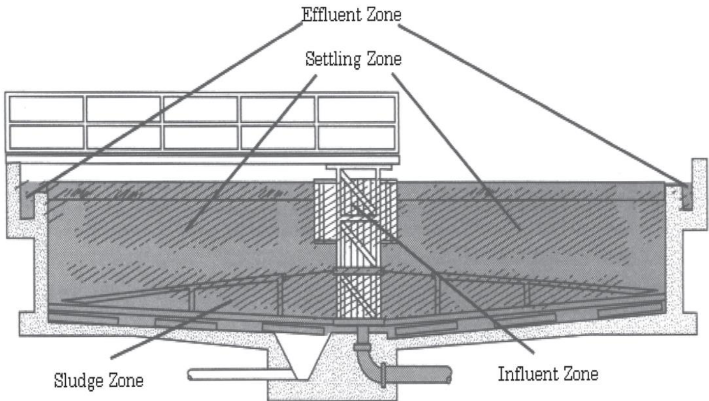
Figure 12.12 - Four Zones of a Sedimentation Basin
