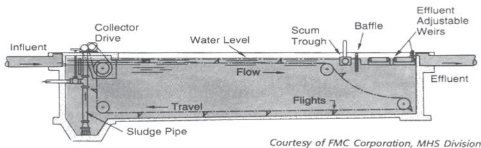
Figure 12.13 - Rectangular Sedimentation Basin
